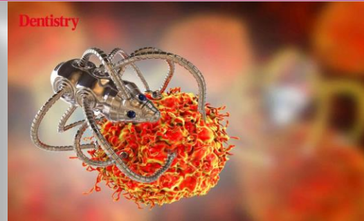
Magnetic nanorobotics
