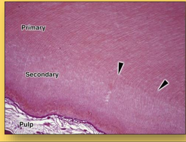
SECONDARY DENTIN
